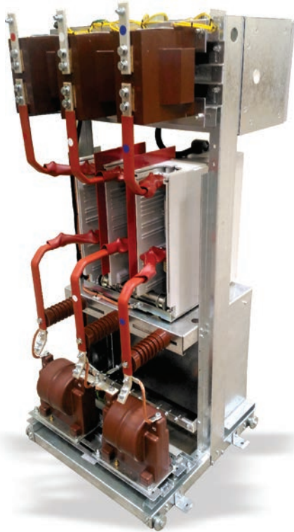
Rear view: Medium Voltage, TC, Circuit breaker and TP.
